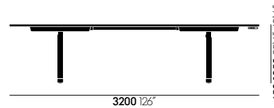
Tyde sit-stand meeting table 320 x 140, rectangular
