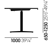
Tyde sit-stand meeting table 200 x 100, rectangular
